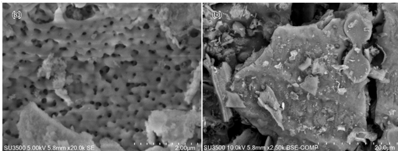
Fig. 3. SEM micrograph of synthesized ZnO@SiO 2 , (a) 20,000 X, and (b) 2,500 X magnifications
