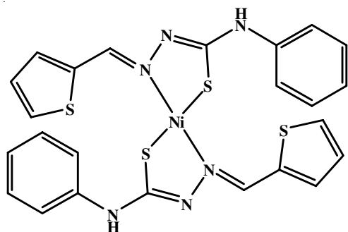
Fig. 15. Structure of Ni(II) complex of 2-thiophene N(4)-phenylthiosemicarbazone
