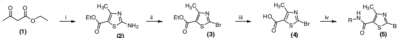
Scheme-I: Synthesis of 2-bromo-4-methylthiazole-5-carboxamide derivatives ( 5a-o ) (i) NBS, thiourea, H 2 O, r.t. (ii) a. conc H 3 PO 4 , conc. H 2 SO 4 , aq. NaNO 2 , 0-5 °C, b. aq. CuBr 2 0-5 °C (iii) 5 % NaOH, r.t. (iv) HATU, RNH 2 , DIPEA, PEG-400, 0 °C → r.t.
