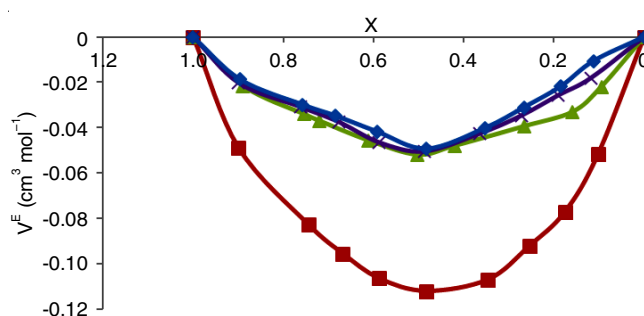
Fig. 1. Curves of V_m^E against X_i for the binary mixtures of THFA + methanoic acid (■), ethanoic acid (▲), propanoic acid (×) and butyric acid (◆) at 298.15 K
